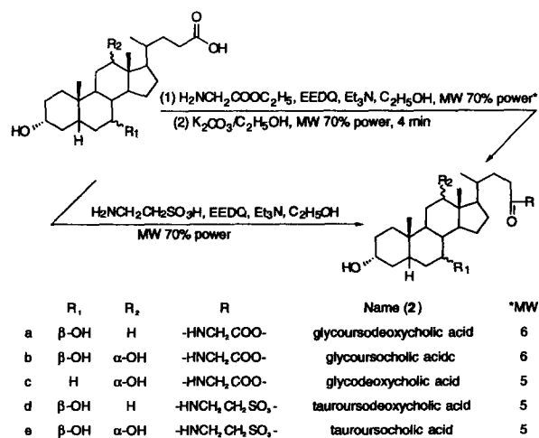
Scheme 1. Conjugation of bile acids with glycine and taurine.
