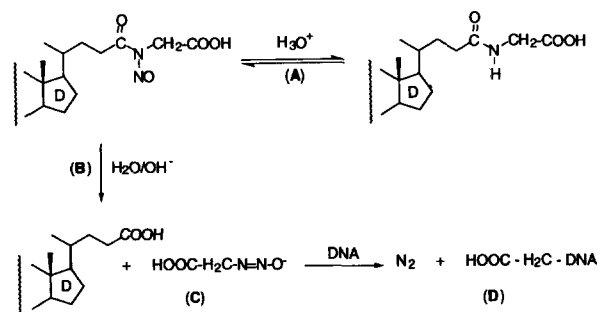
Scheme 3. Decomposition of N -nitroso glyco-bile acid conjugates.
