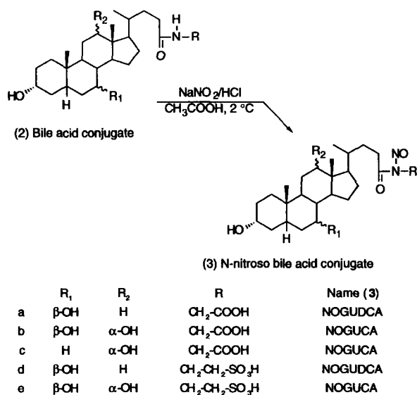
Scheme 2. N -nitrosation of bile acid conjugates.
